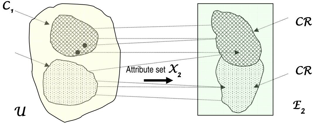
Figure 6: A homomorphic attribute set \mathcal{X}_2 spanning an inconsistent instance space.
