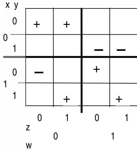
a) Visualization of training data
