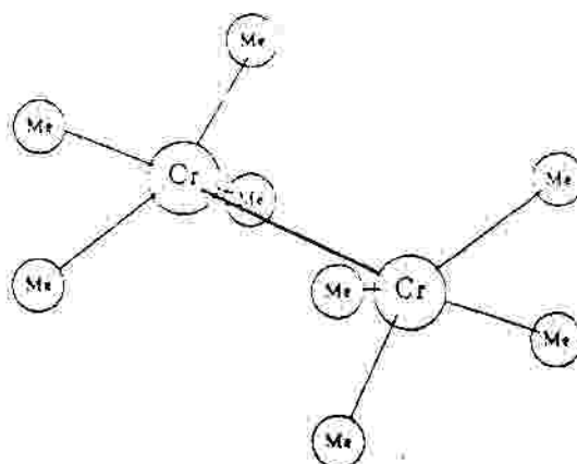
Figure 6-8: Bimetallic coordination compound in eclipsed conformation
