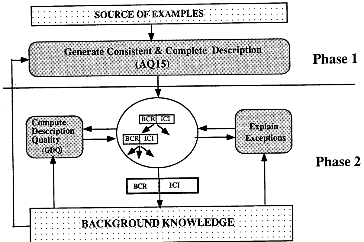
Figure 1. Learning in the POSEIDON system
