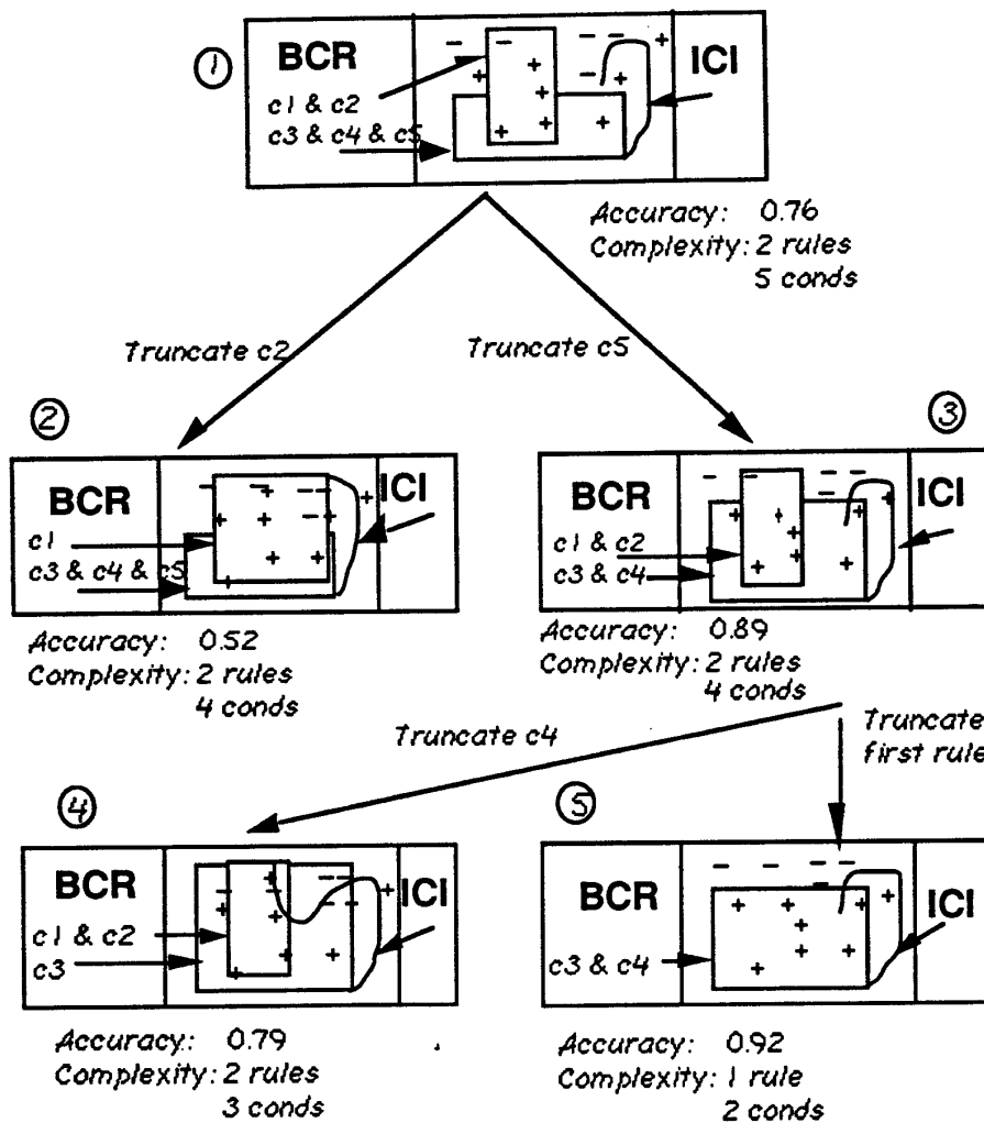
Figure 2. An illustration of the search process.
