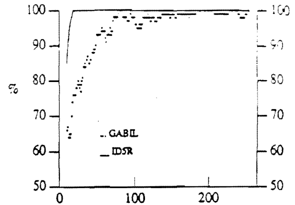
Instances Processed Fig 1. 1D1C
