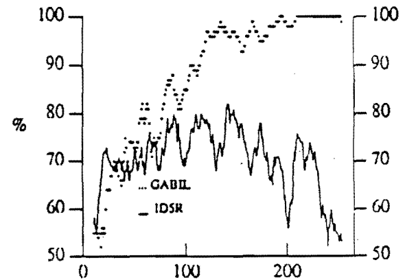
Instances Processed Fig 2. 4D1C
