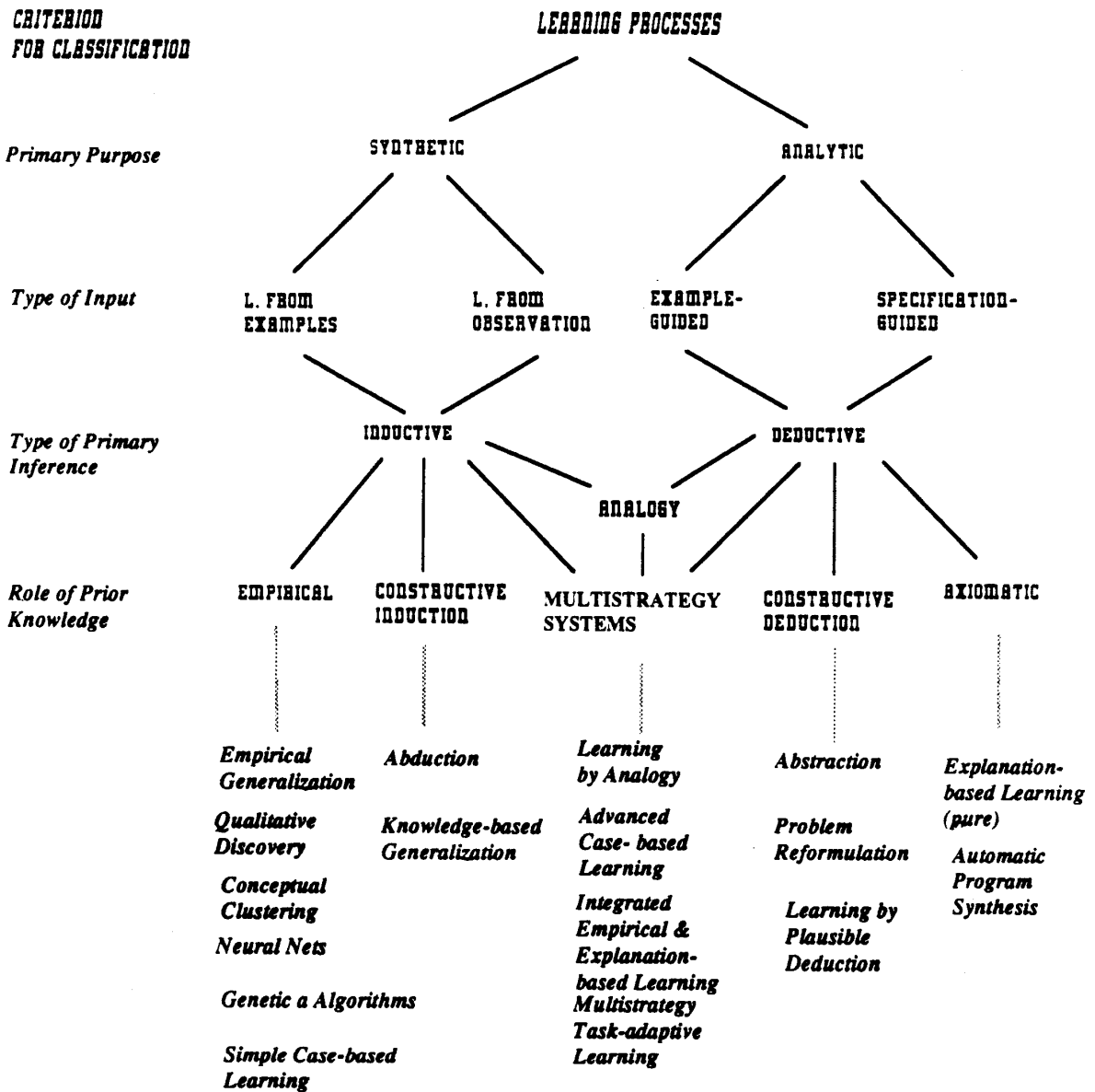
Figure 4. A general classification of learning processes.
