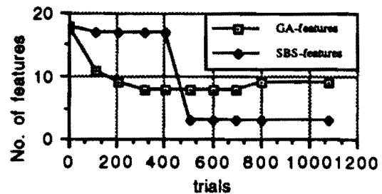
Figure 7: The number of features used by the best individual
