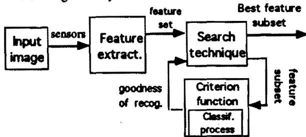
Figure 1: Block diagram of the adaptive feature selection process
