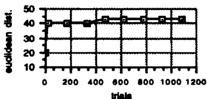
Figure 3: The improvement of Euclidean distance measure over time
