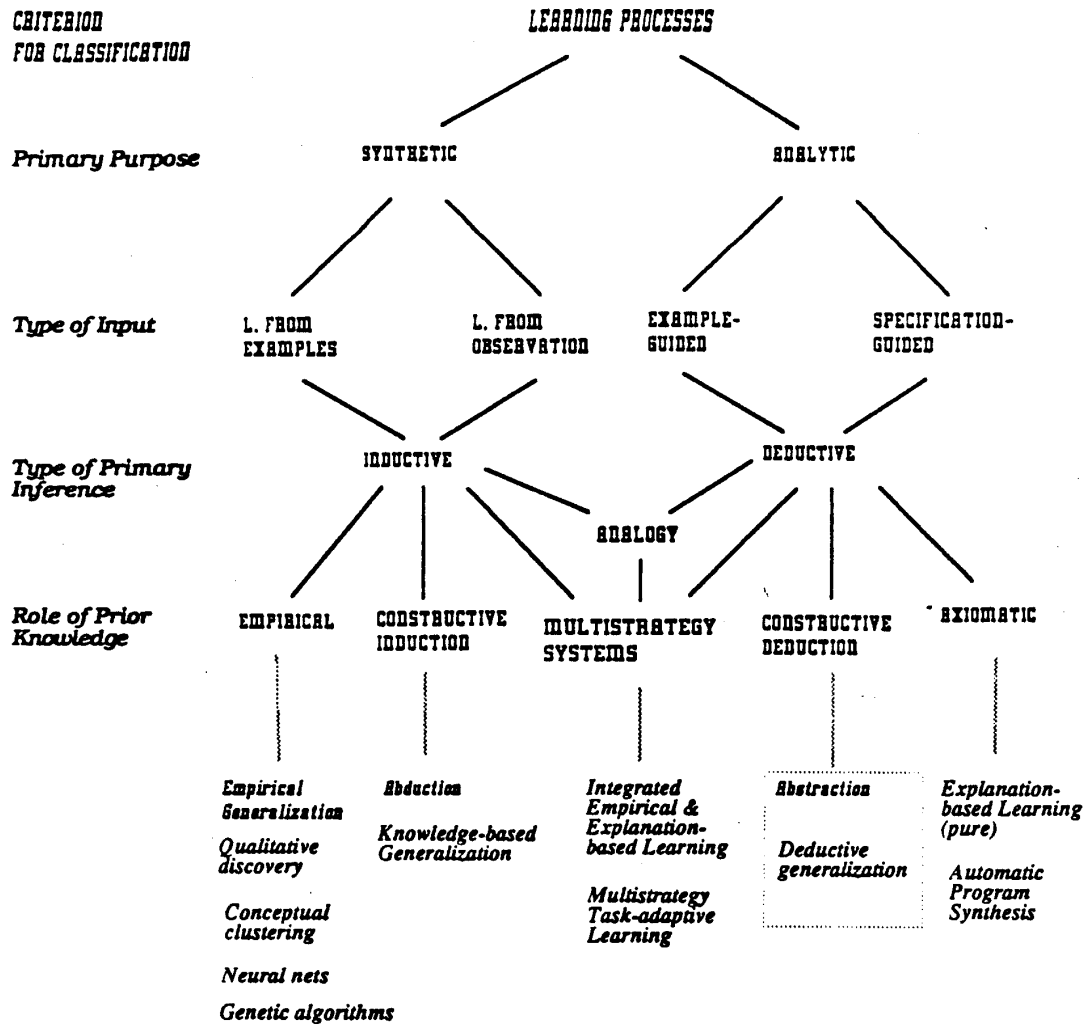
Figure 2. A multicriterion classification of learning processes.
