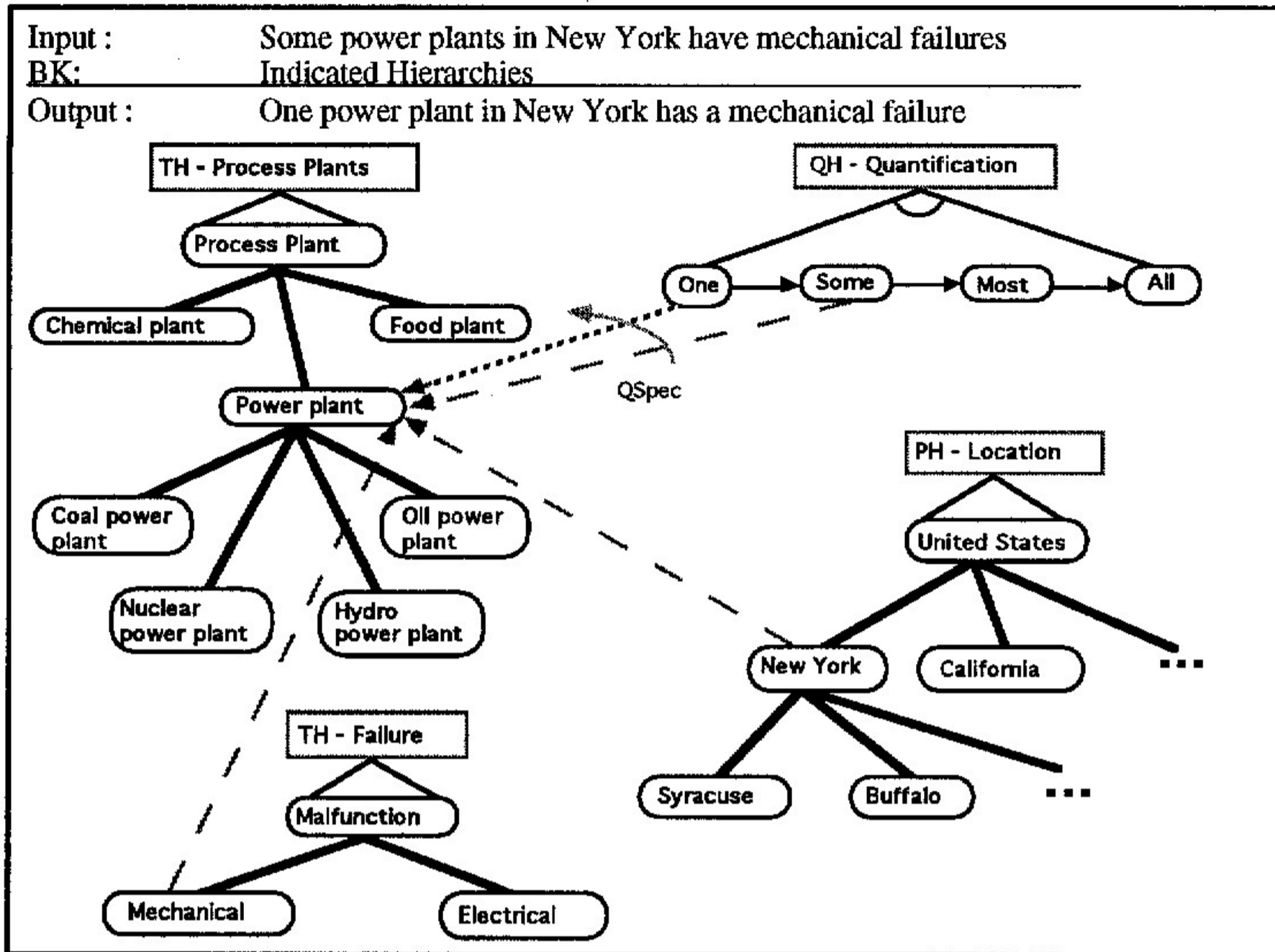
Figure 6: Deductive specialization based on quantification.
