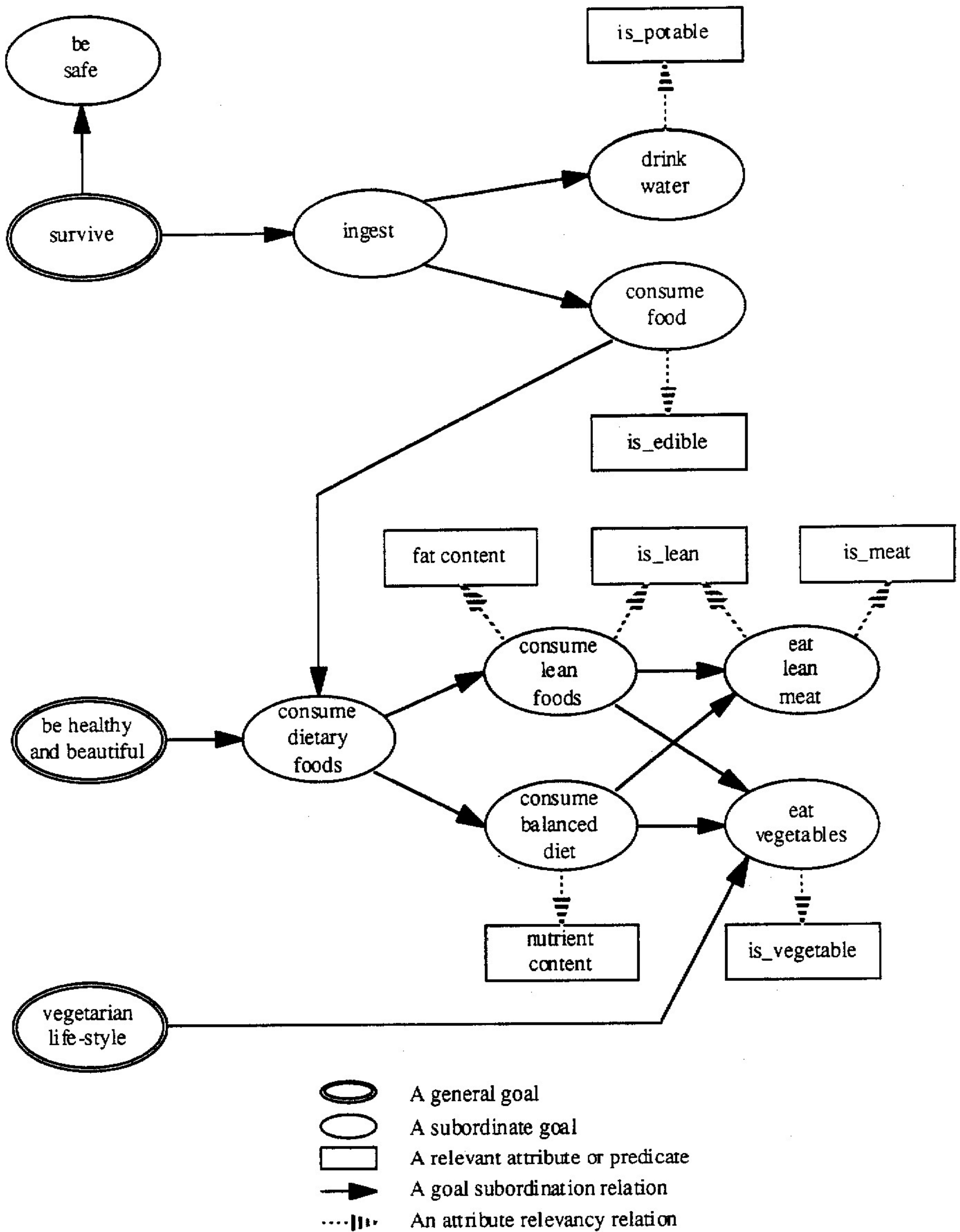
Figure 2: An example goal dependency network for the goals to survive, to be healthy, and to live a vegetarian life-style.
