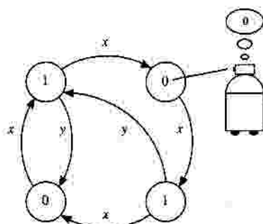
Figure 12. Automaton representation of a dynamical system.
