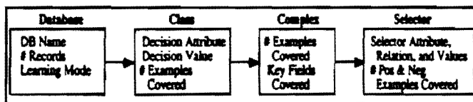
Figure 3: Knowledge segment components
