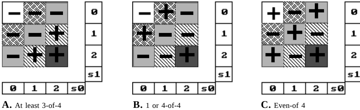
Figure 12. Transformation replacing AND and XOR with ADD. The concepts are symmetrical with respect to attributes s0 and s1 . The shaded areas mark XOR symmetries in this representation space.
