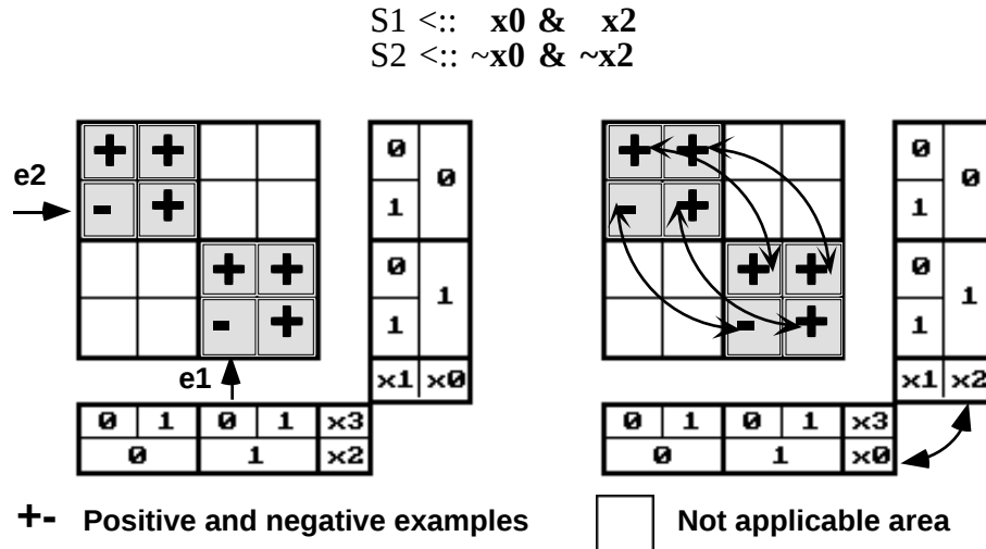
Figure 1. Equivalence symmetry with respect to attributes x0 and x2
