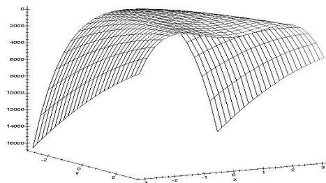
Figure 5. An inverted graph of a two-dimensional projection of the Rosenbrock function.
