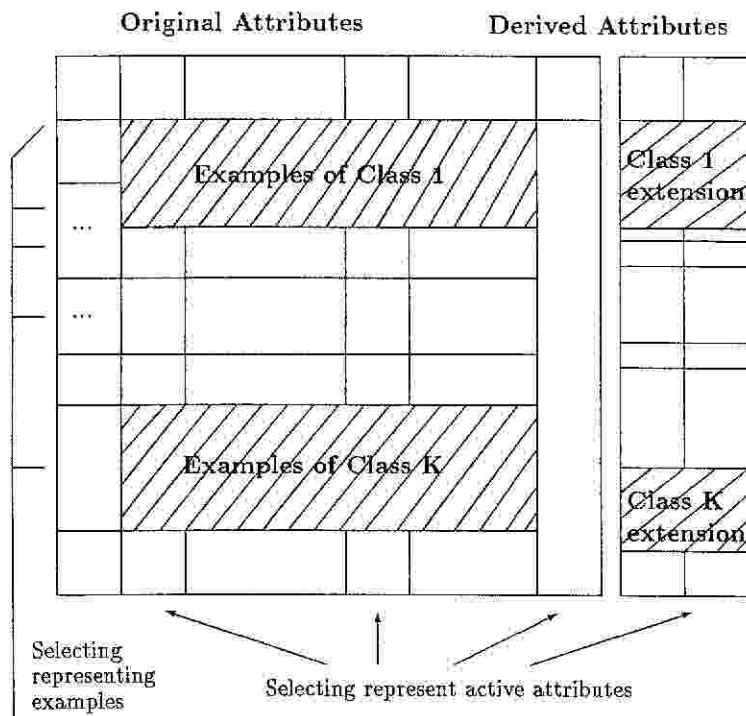
Figure 3. An illustration of the role of different knowledge generation operators
