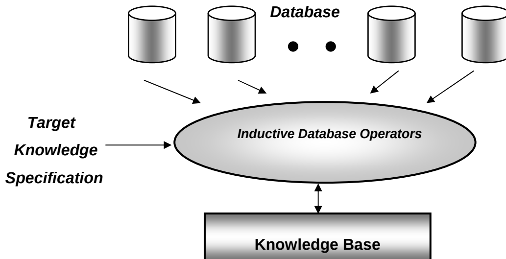
Figure 1. A general diagram of an inductive database.
