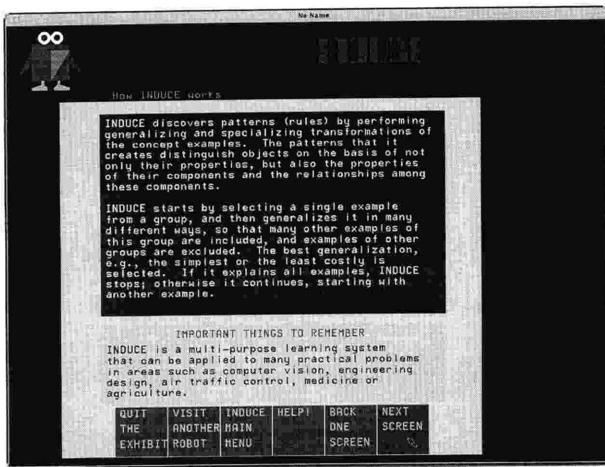
Figure 8. INDUCE's Capabilities
