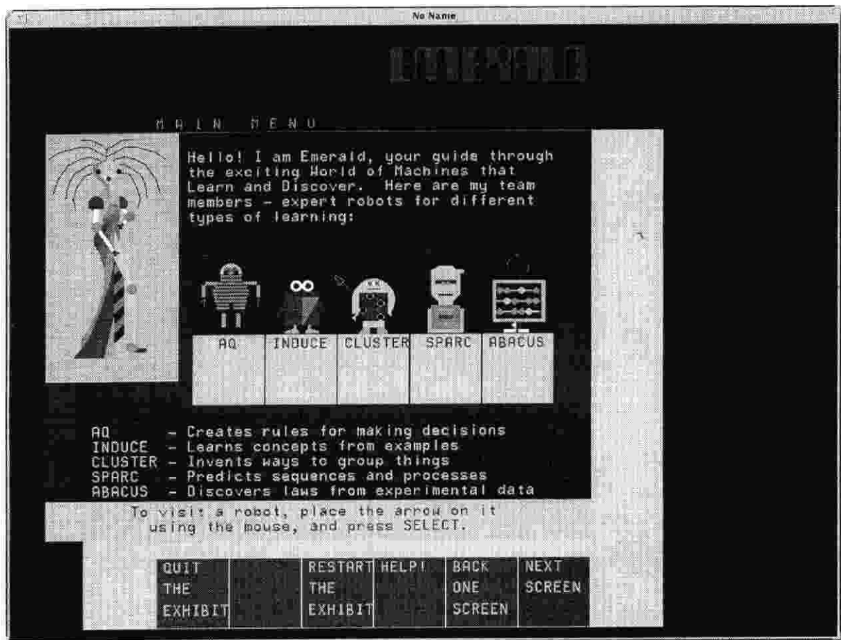
Figure 2. Main Menu
