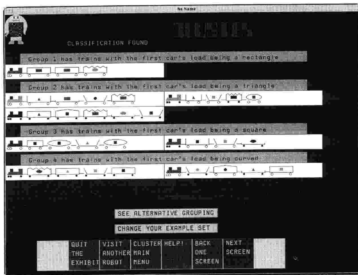
Figure 11. CLUSTER's Classification
